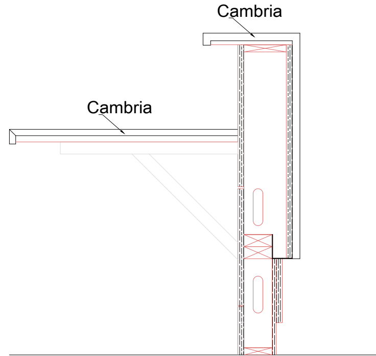
RECEPTION DESK SECTION: AA
